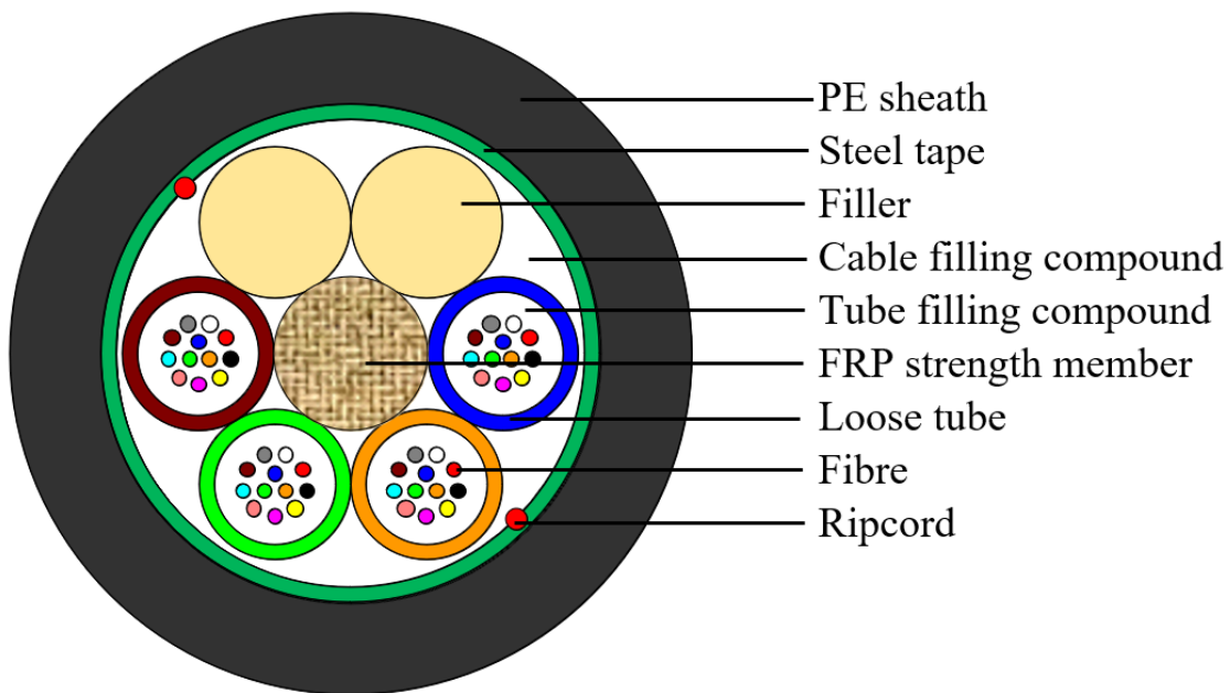
GYFTS-48B1.3 Schematic for reference only
